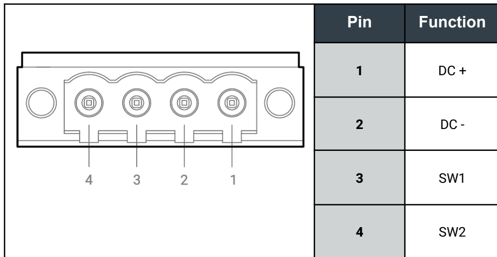
Terminal block power pinout
