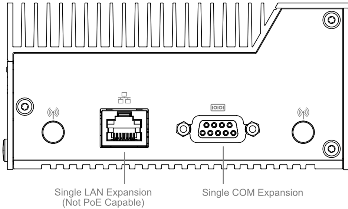
K430 Top I/O LAN / COM Expansion.
